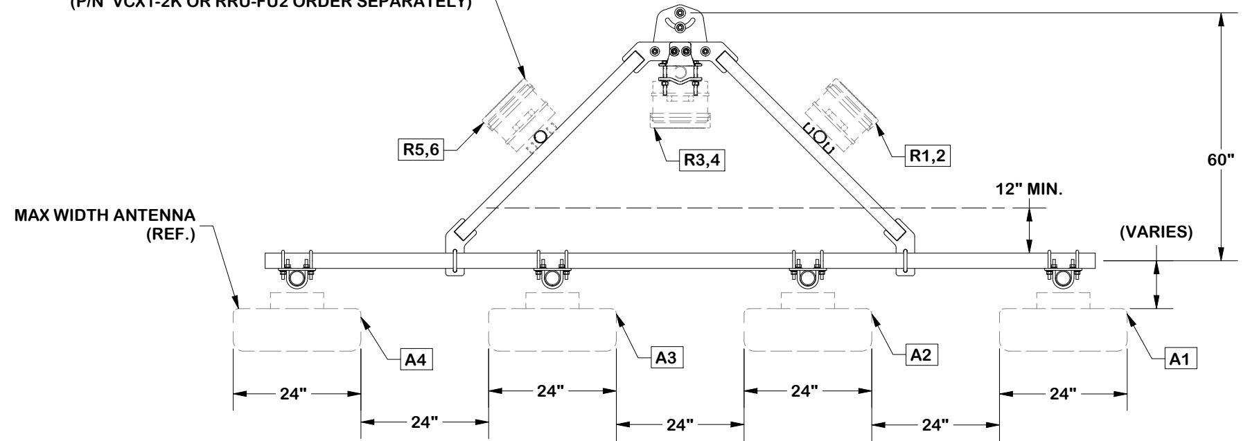
TOP VIEW
